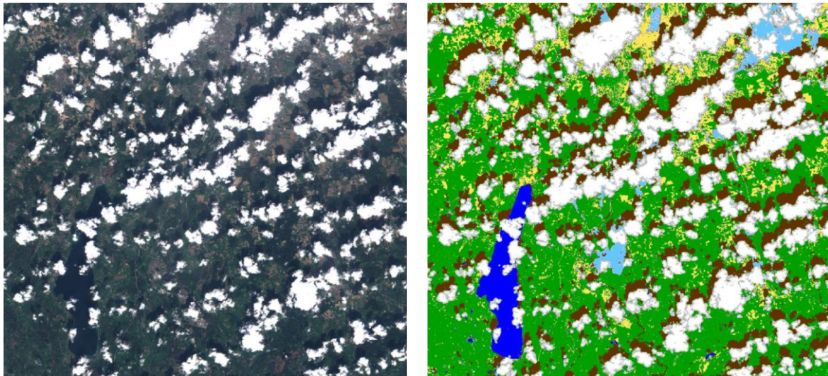
Figure 2-6 – L1C True Colour Image (TCI), L2A Scene Classification (SCL)
